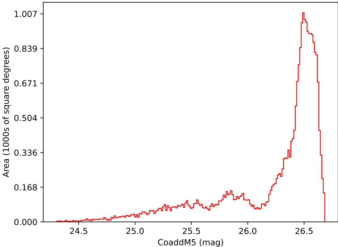
too_elab_r128_d3_ugrizy_v3.4_10yrs All sky i band: CoaddM5
