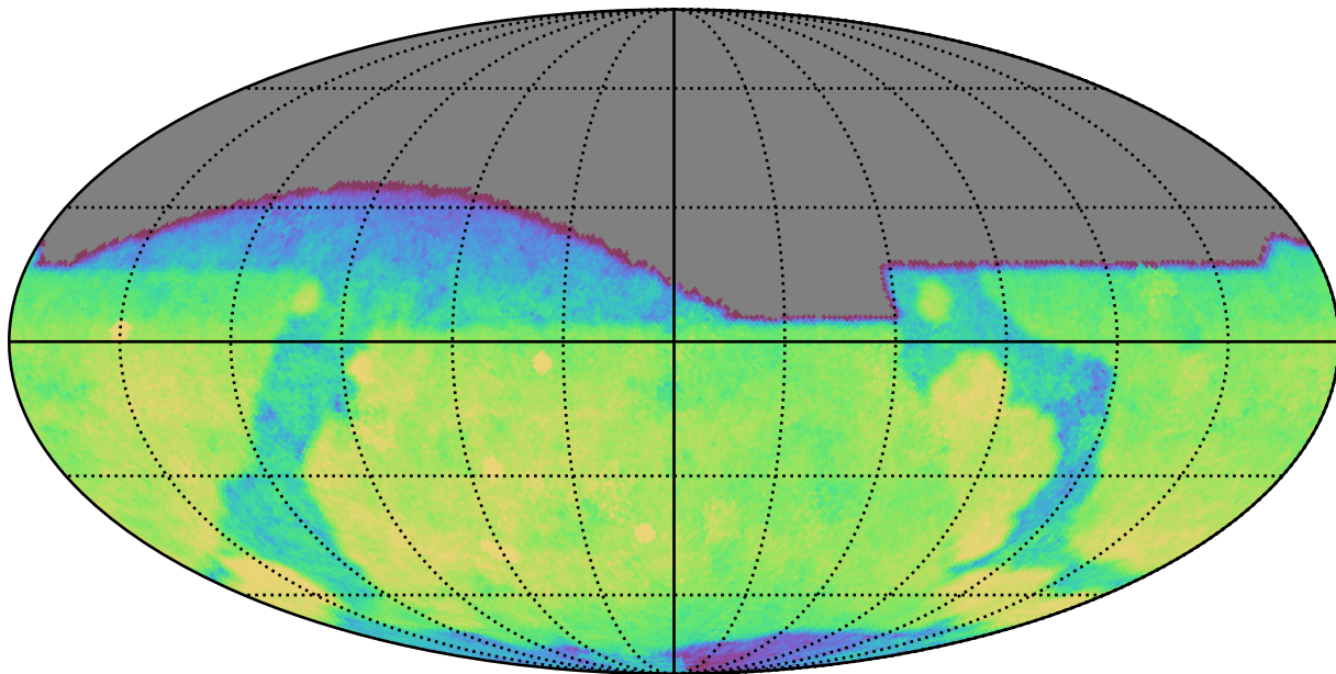
too_elab_r128_d3_ugrizy_v3.4_10yrs All sky g band: CoaddM5
