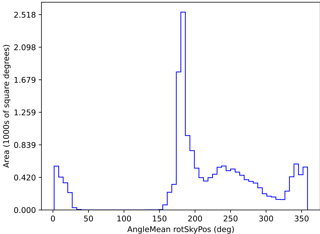
too_elab_r128_d3_ugrizy_v3.4_10yrs WFD all bands: AngleMean rotSkyPos
