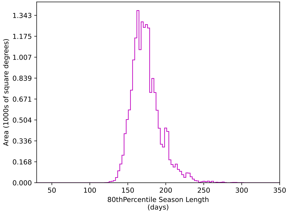
too_elab_r128_d3_ugrizy_v3.4_10yrs WFD z band: 80thPercentile Season Length
