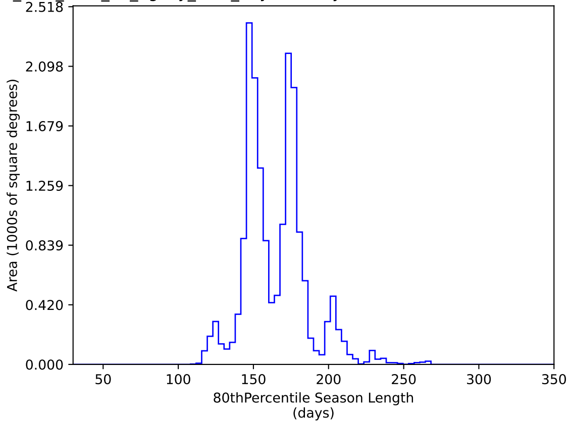
too_elab_r128_d3_ugrizy_v3.4_10yrs WFD y band: 80thPercentile Season Length
