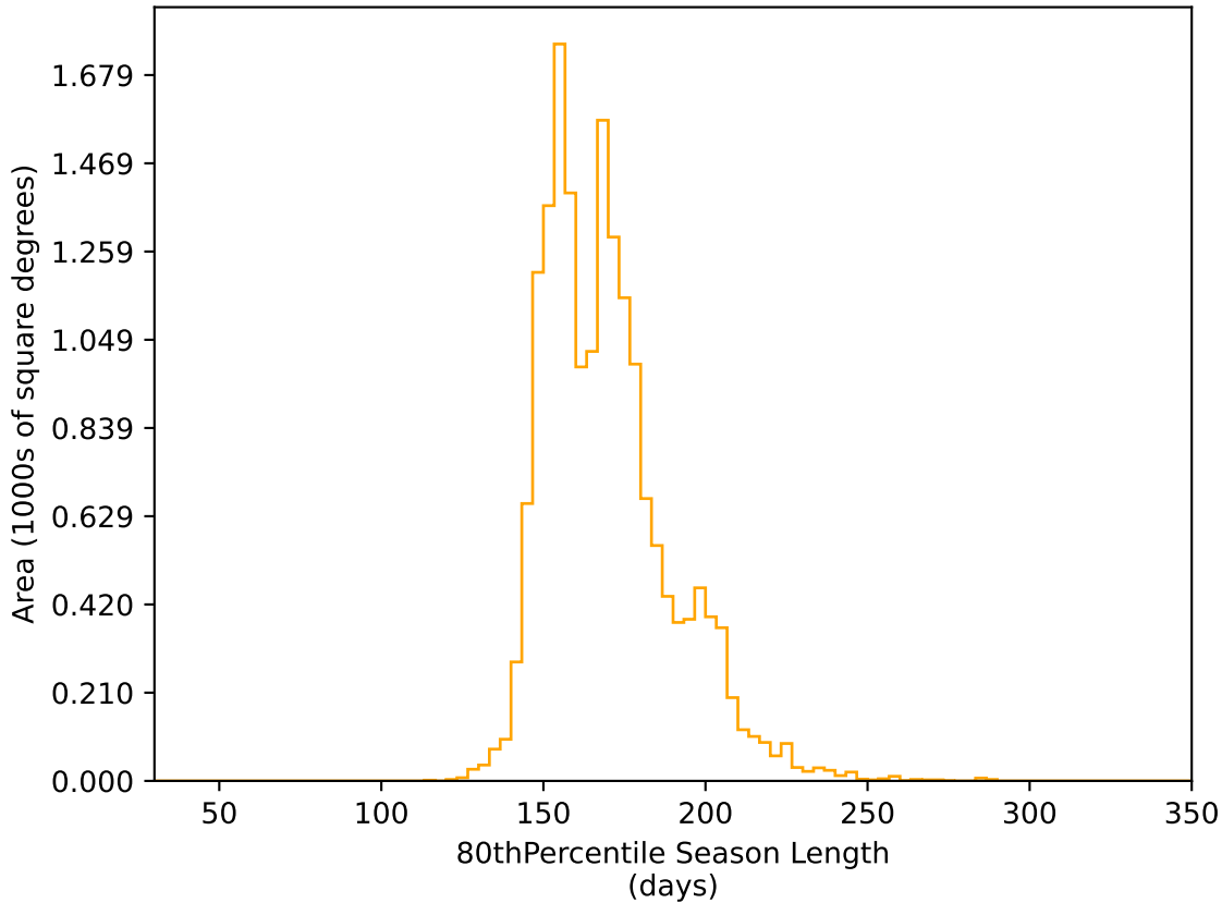
too_elab_r128_d3_ugrizy_v3.4_10yrs WFD r band: 80thPercentile Season Length
