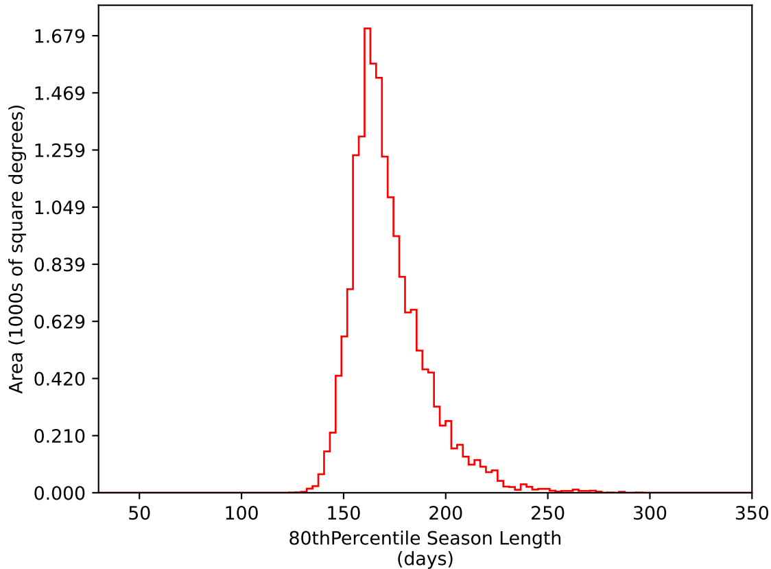
too_elab_r128_d3_ugrizy_v3.4_10yrs WFD i band: 80thPercentile Season Length
