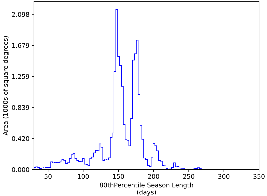
too_elab_r128_d3_ugrizy_v3.4_10yrs All sky y band: 80thPercentile Season Length
