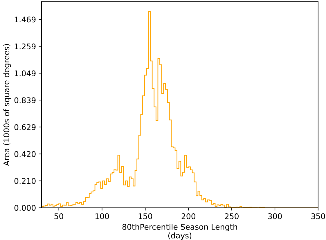
too_elab_r128_d3_ugrizy_v3.4_10yrs All sky r band: 80thPercentile Season Length
