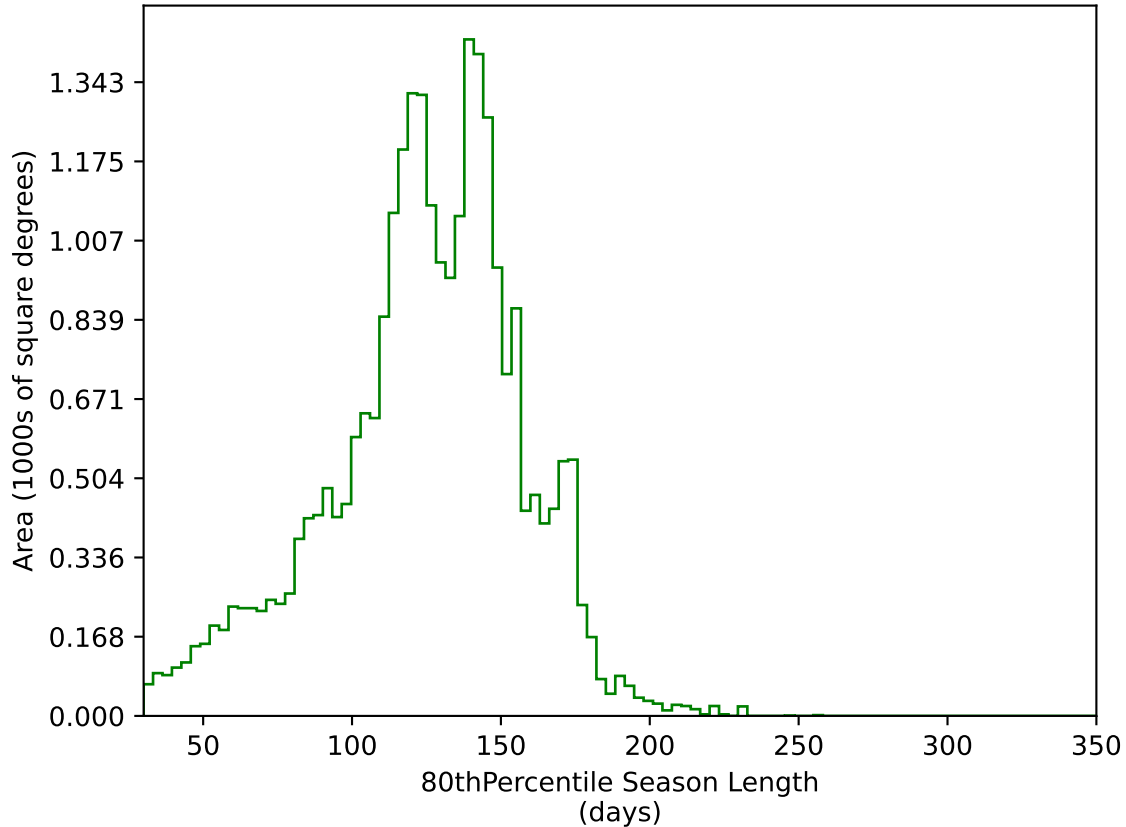
too_elab_r128_d3_ugrizy_v3.4_10yrs All sky g band: 80thPercentile Season Length
