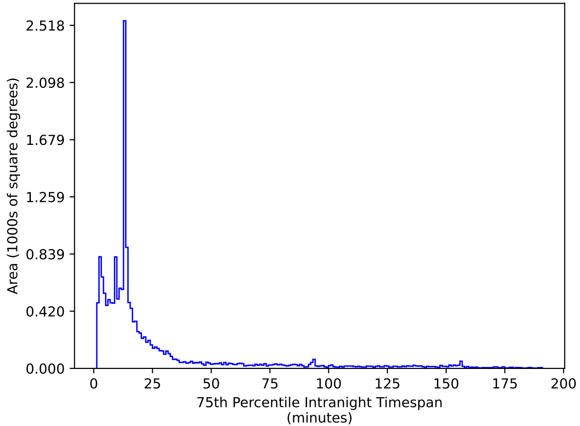
too_elab_r128_d3_ugrizy_v3.4_10yrs WFD z band: 75th Percentile Intranight Timespan
