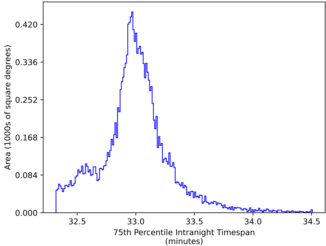
too_elab_r128_d3_ugrizy_v3.4_10yrs WFD y band: 75th Percentile Intranight Timespan
