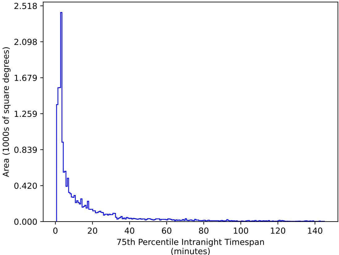
too_elab_r128_d3_ugrizy_v3.4_10yrs WFD g band: 75th Percentile Intranight Timespan
