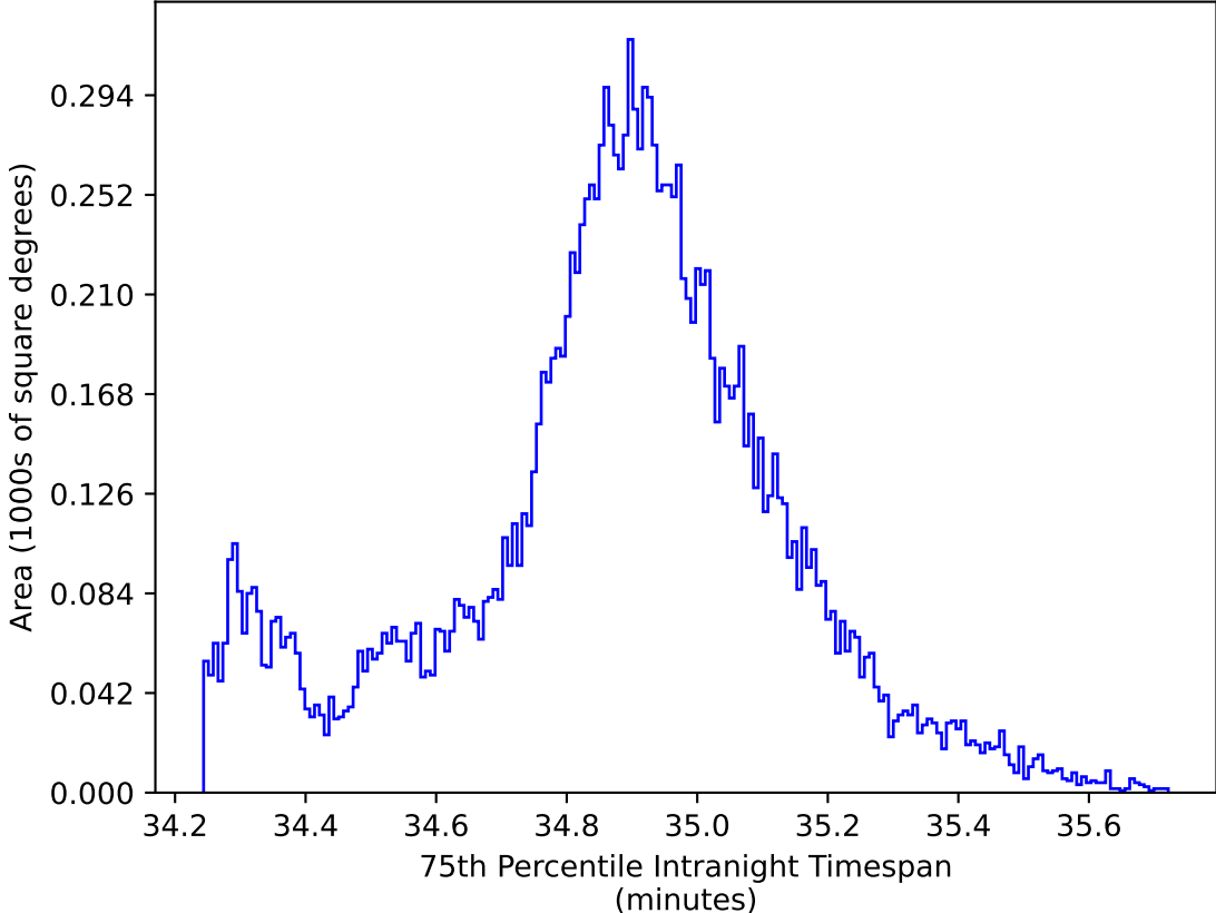
too_elab_r128_d3_ugrizy_v3.4_10yrs WFD all bands: 75th Percentile Intranight Timespan
