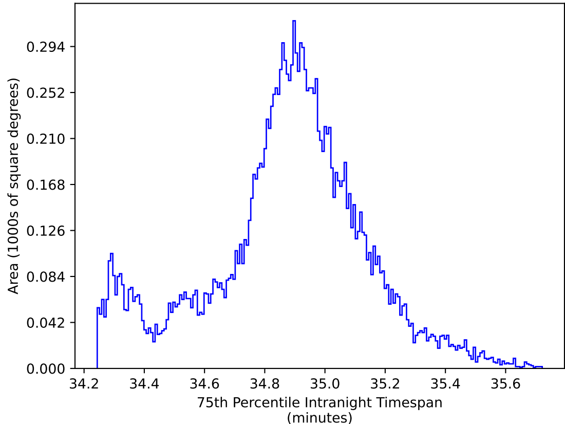
too_elab_r128_d3_ugrizy_v3.4_10yrs WFD: 75th Percentile Intranight Timespan
