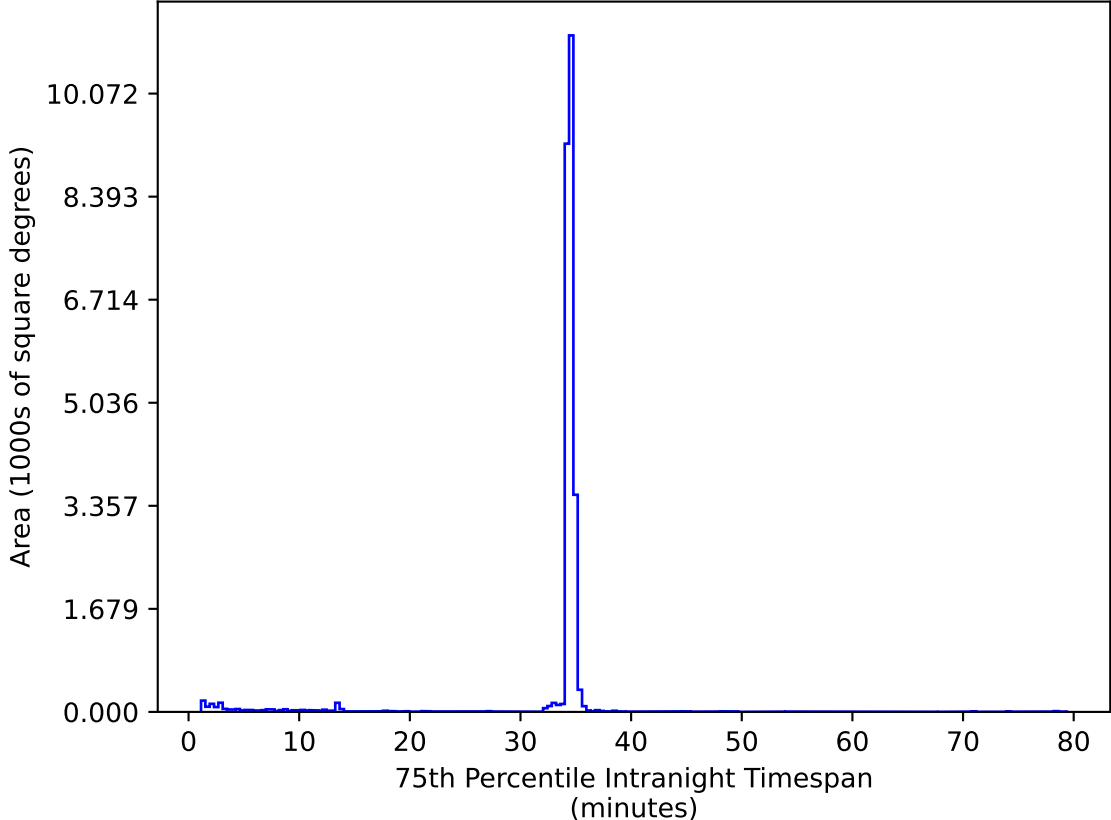
too_elab_r128_d3_ugrizy_v3.4_10yrs All sky zy bands: 75th Percentile Intranight Timespan
