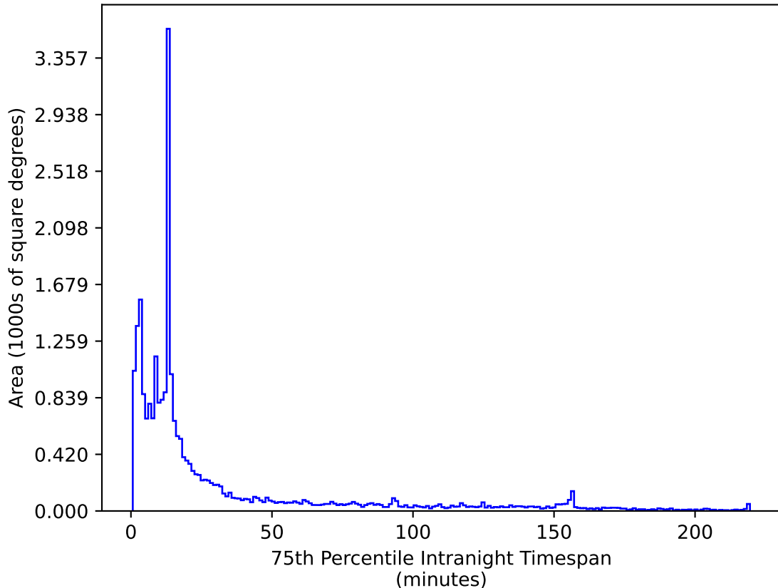
too_elab_r128_d3_ugrizy_v3.4_10yrs All sky z band: 75th Percentile Intranight Timespan
