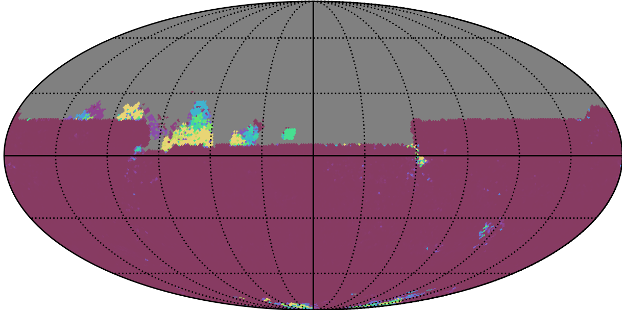
too_elab_r128_d3_ugrizy_v3.4_10yrs All sky y band: 75th Percentile Intranight Timespan
