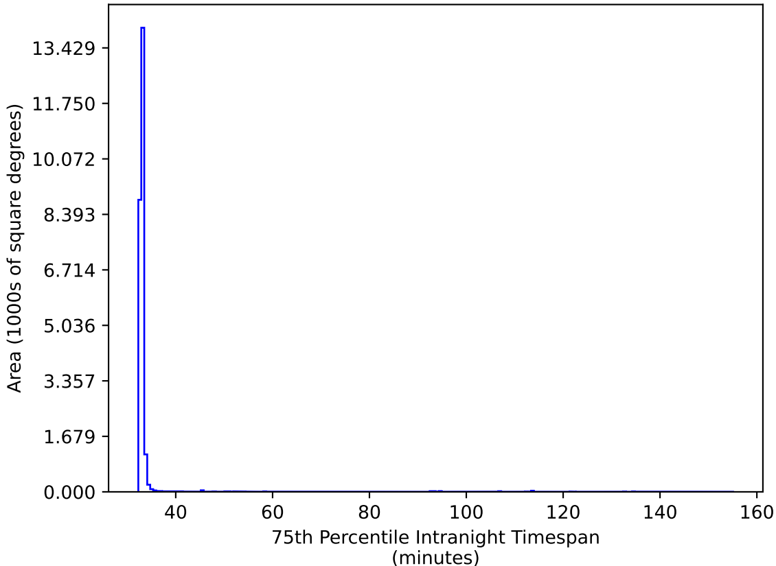
too_elab_r128_d3_ugrizy_v3.4_10yrs All sky y band: 75th Percentile Intranight Timespan
