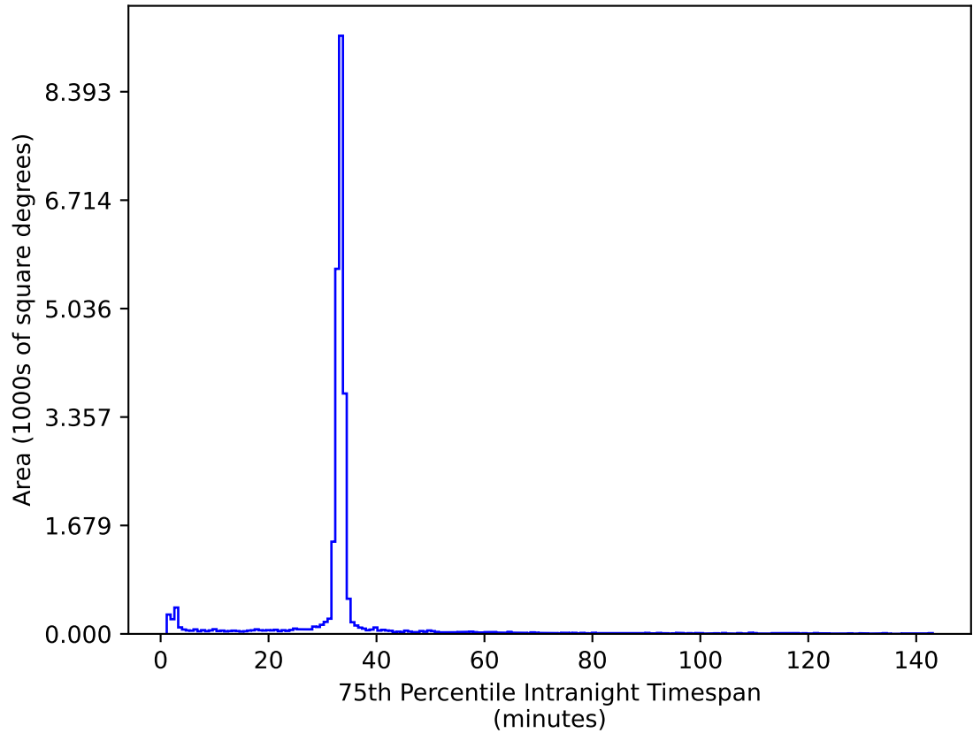
too_elab_r128_d3_ugrizy_v3.4_10yrs All sky ug bands: 75th Percentile Intranight Timespan
