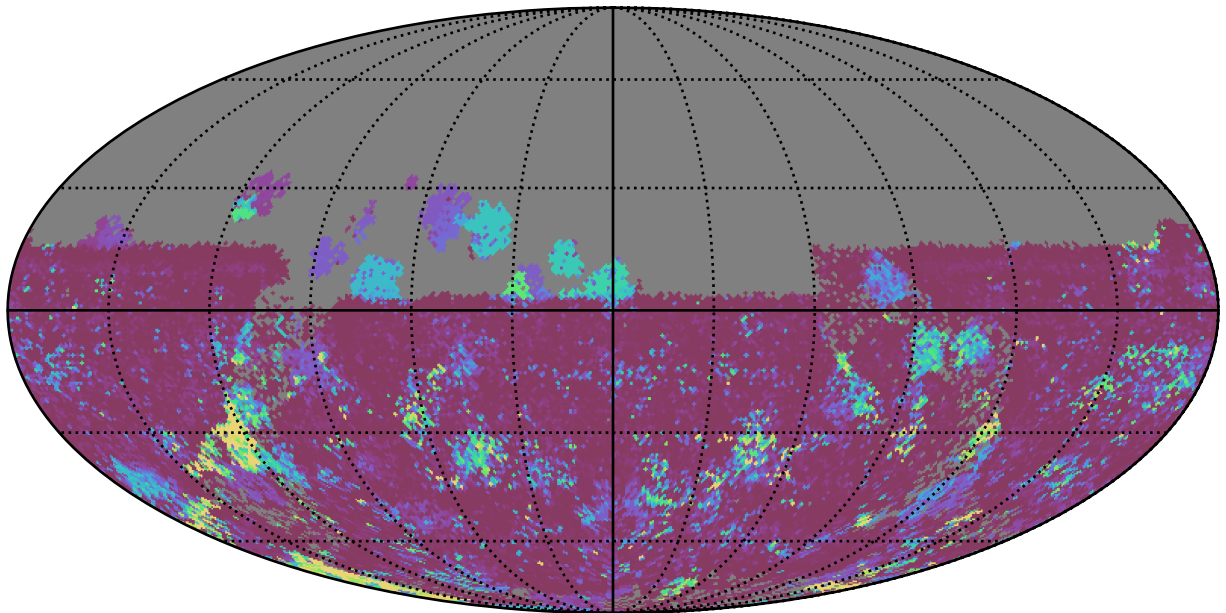
too_elab_r128_d3_ugrizy_v3.4_10yrs All sky u band: 75th Percentile Intranight Timespan
