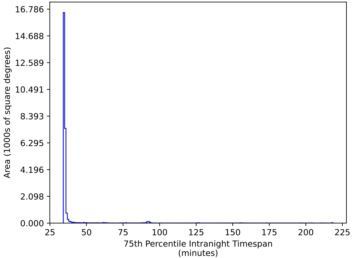
too_elab_r128_d3_ugrizy_v3.4_10yrs All sky ri bands: 75th Percentile Intranight Timespan
