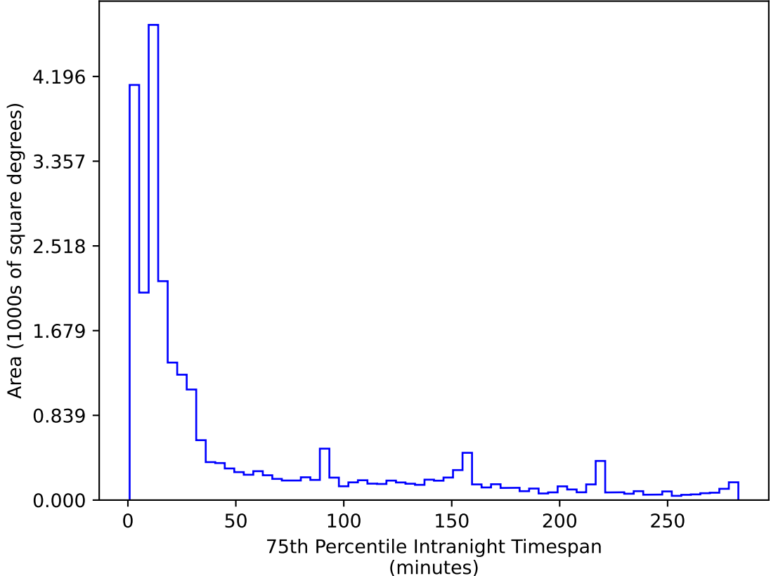
too_elab_r128_d3_ugrizy_v3.4_10yrs All sky r band: 75th Percentile Intranight Timespan
