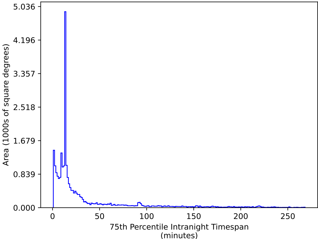
too_elab_r128_d3_ugrizy_v3.4_10yrs All sky i band: 75th Percentile Intranight Timespan
