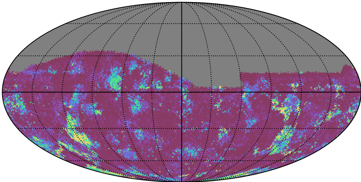
too_elab_r128_d3_ugrizy_v3.4_10yrs All sky g band: 75th Percentile Intranight Timespan
