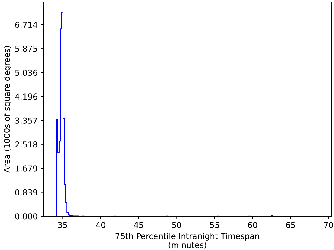
too_elab_r128_d3_ugrizy_v3.4_10yrs All sky all bands: 75th Percentile Intranight Timespan
