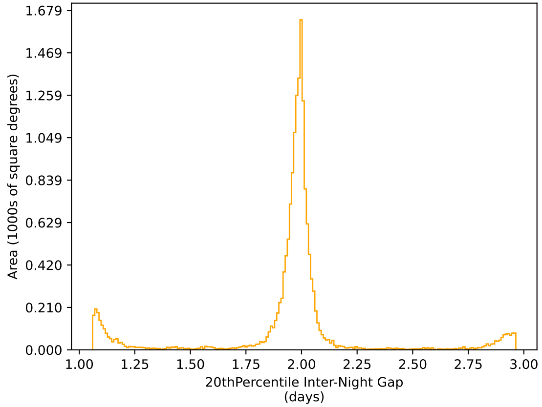
too_elab_r128_d3_ugrizy_v3.4_10yrs WFD r band: 20thPercentile Inter-Night Gap
