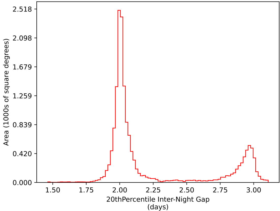
too_elab_r128_d3_ugrizy_v3.4_10yrs WFD i band: 20thPercentile Inter-Night Gap
