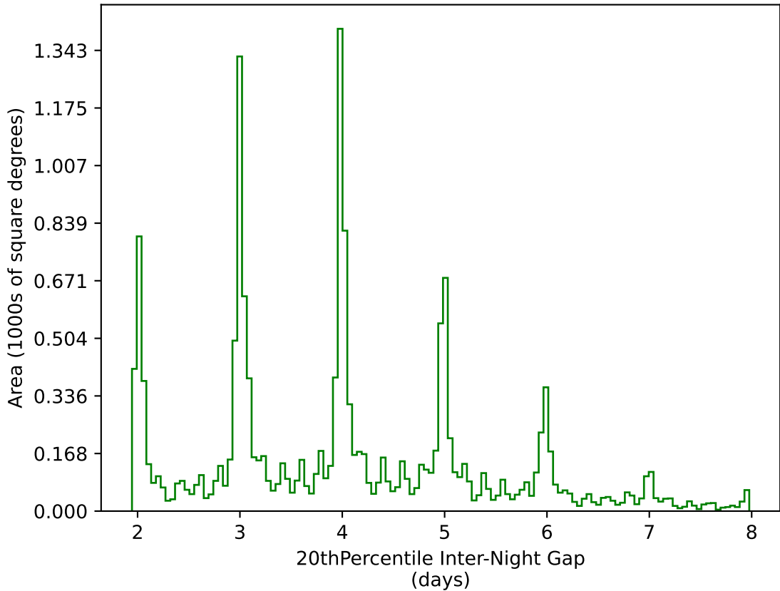
too_elab_r128_d3_ugrizy_v3.4_10yrs WFD g band: 20thPercentile Inter-Night Gap
