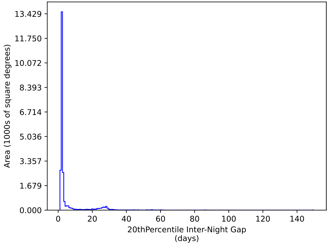
too_elab_r128_d3_ugrizy_v3.4_10yrs All sky y band: 20thPercentile Inter-Night Gap
