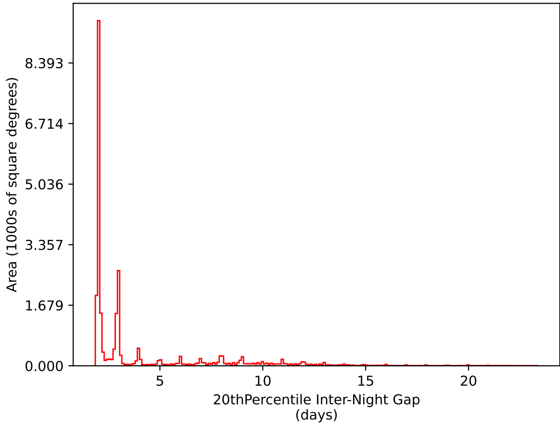
too_elab_r128_d3_ugrizy_v3.4_10yrs All sky i band: 20thPercentile Inter-Night Gap
