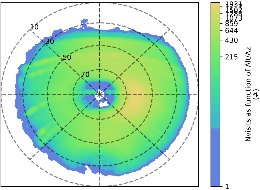
too_elab_r128_d3_ugrizy_v3.4_10yrs y: Nvisits as function of Alt/Az
