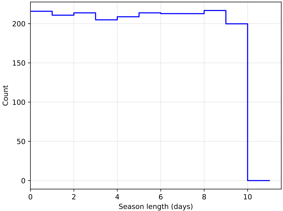
too_elab_r128_d3_ugrizy_v3.4_10yrs DD:ECDFS all bands: SeasonLength
