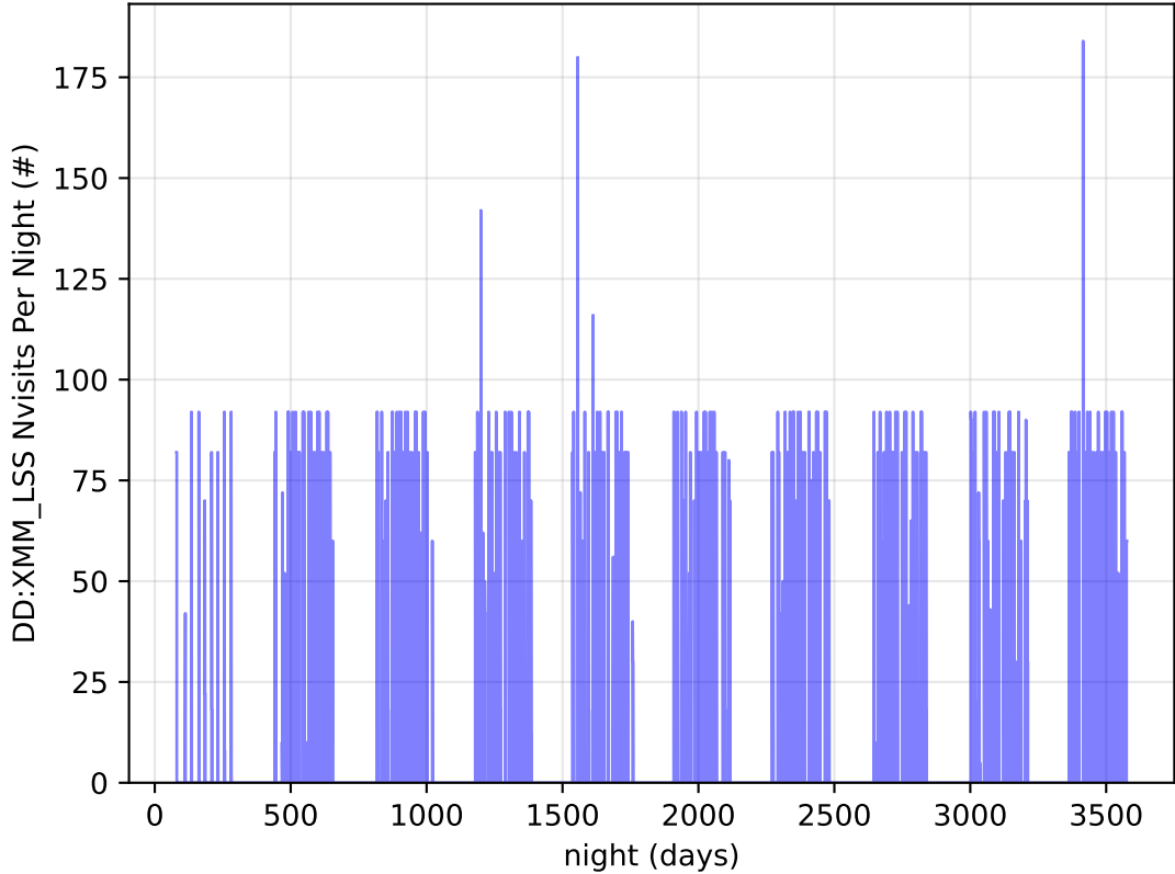
too_elab_r128_d3_ugrizy_v3.4_10yrs all bands: DD:XMM_LSS Nvisits Per Night
