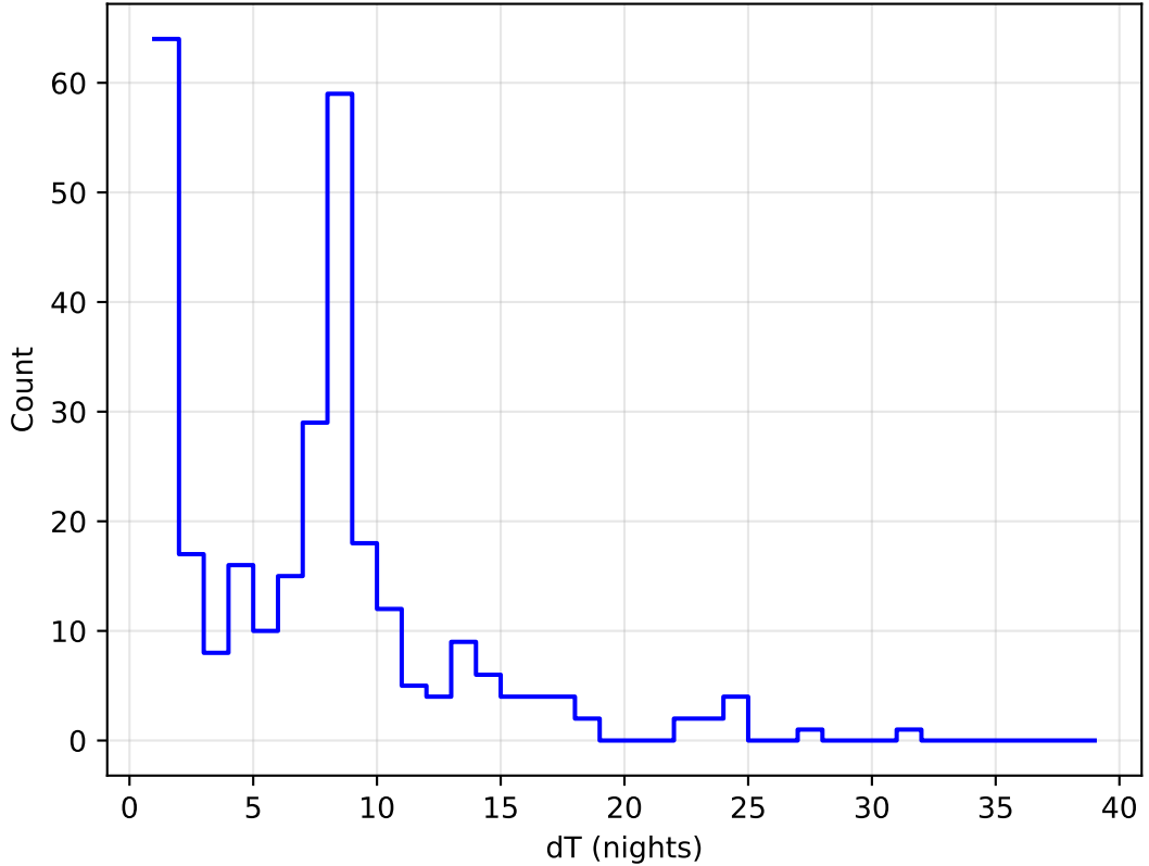
too_elab_r128_d3_ugrizy_v3.4_10yrs all bands: DD:XMM_LSS Delta Nights Histogram
