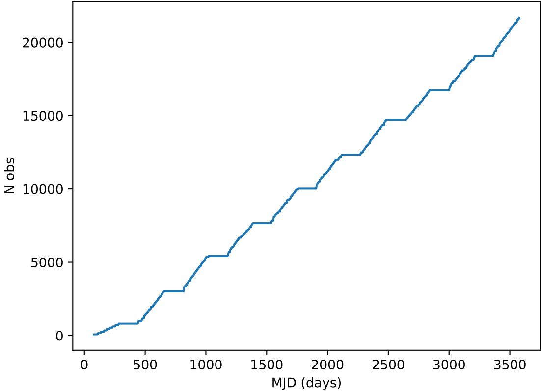
too_elab_r128_d3_ugrizy_v3.4_10yrs all bands: DD:XMM_LSS Cumulative NVisits
