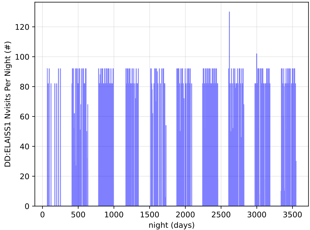
too_elab_r128_d3_ugrizy_v3.4_10yrs all bands: DD:ELAISS1 Nvisits Per Night
