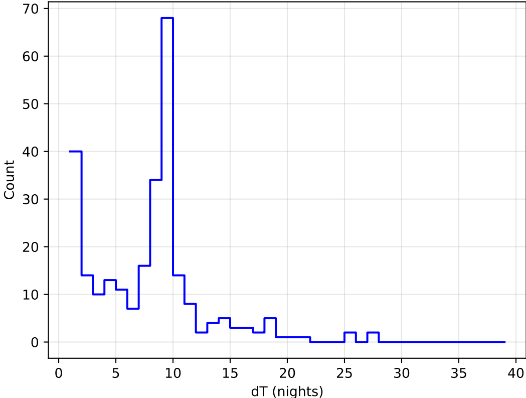
too_elab_r128_d3_ugrizy_v3.4_10yrs all bands: DD:ELAISS1 Delta Nights Histogram
