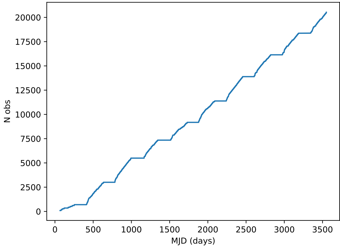
too_elab_r128_d3_ugrizy_v3.4_10yrs all bands: DD:ELAISS1 Cumulative NVisits
