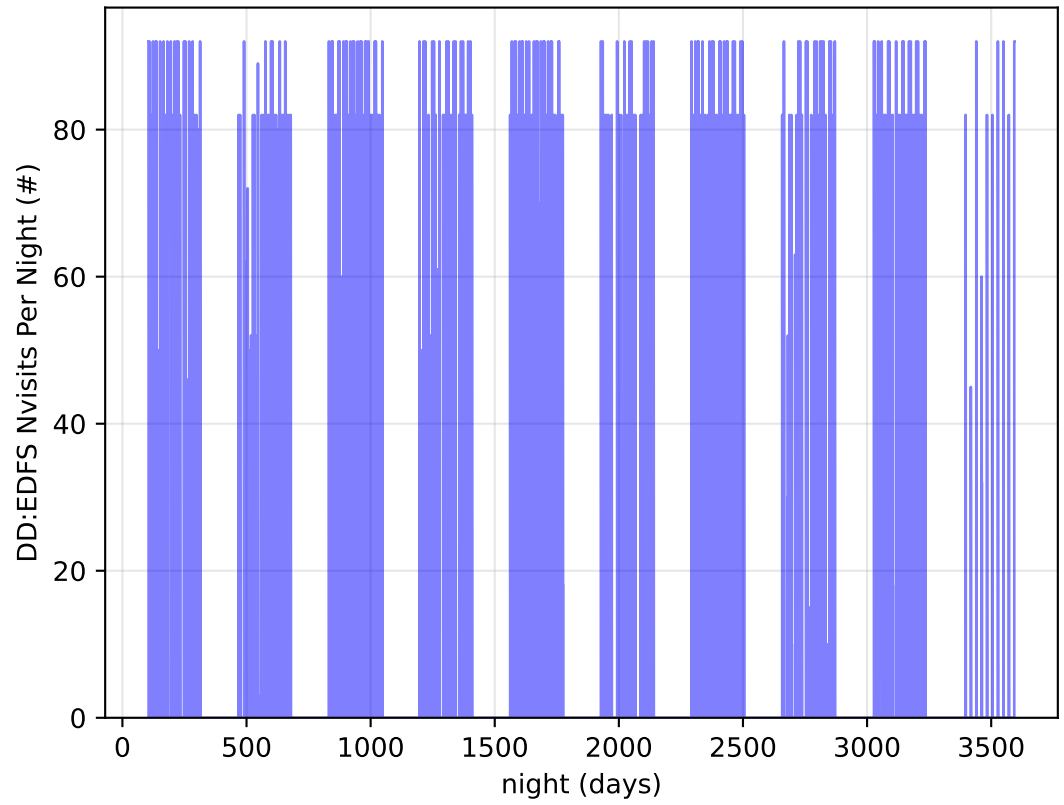
too_elab_r128_d3_ugrizy_v3.4_10yrs all bands: DD:EDFS Nvisits Per Night
