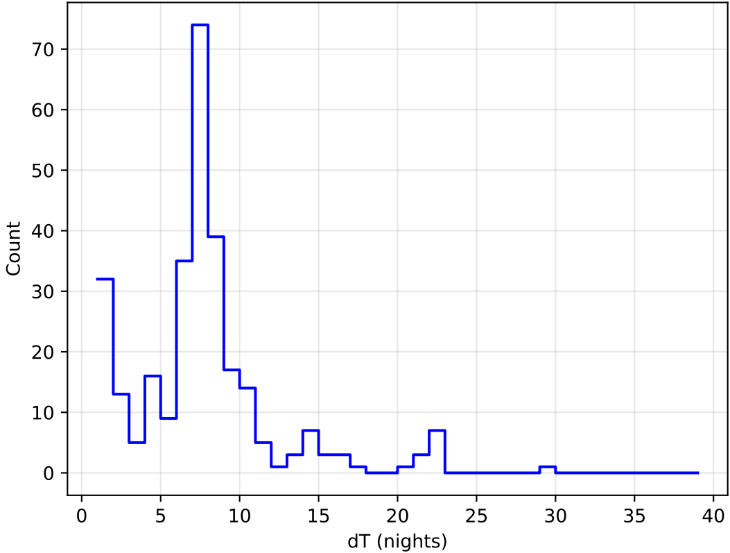
too_elab_r128_d3_ugrizy_v3.4_10yrs all bands: DD:EDFS Delta Nights Histogram
