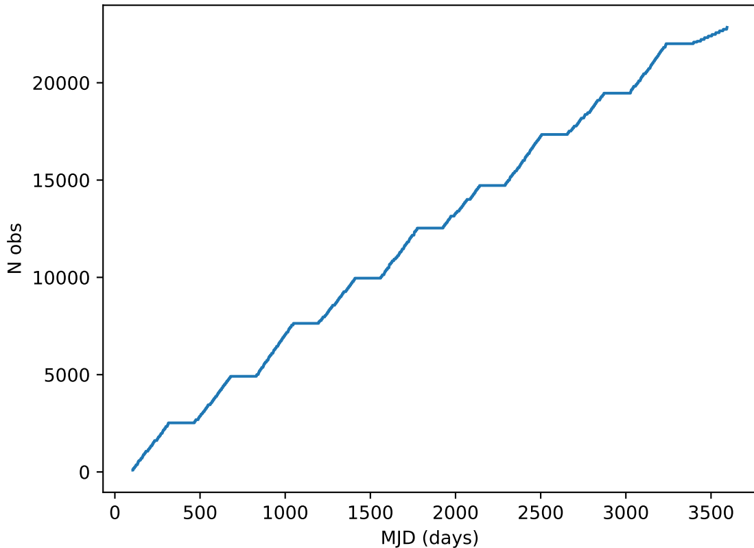
too_elab_r128_d3_ugrizy_v3.4_10yrs all bands: DD:EDFS Cumulative NVisits
