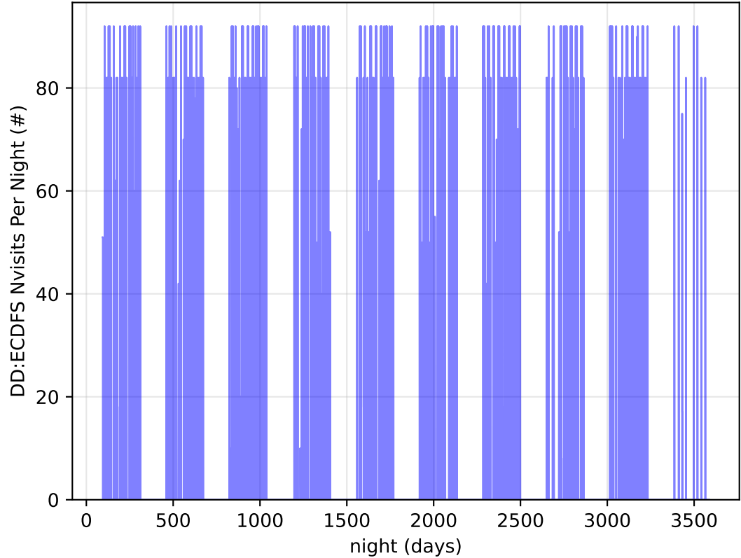
too_elab_r128_d3_ugrizy_v3.4_10yrs all bands: DD:ECDFS Nvisits Per Night
