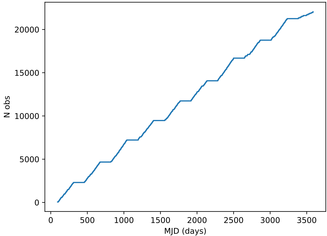
too_elab_r128_d3_ugrizy_v3.4_10yrs all bands: DD:ECDFS Cumulative NVisits
