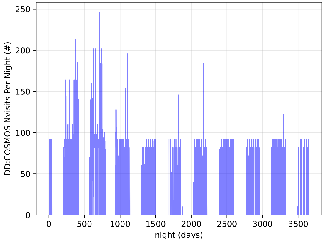
too_elab_r128_d3_ugrizy_v3.4_10yrs all bands: DD: COSMOS Nvisits Per Night
