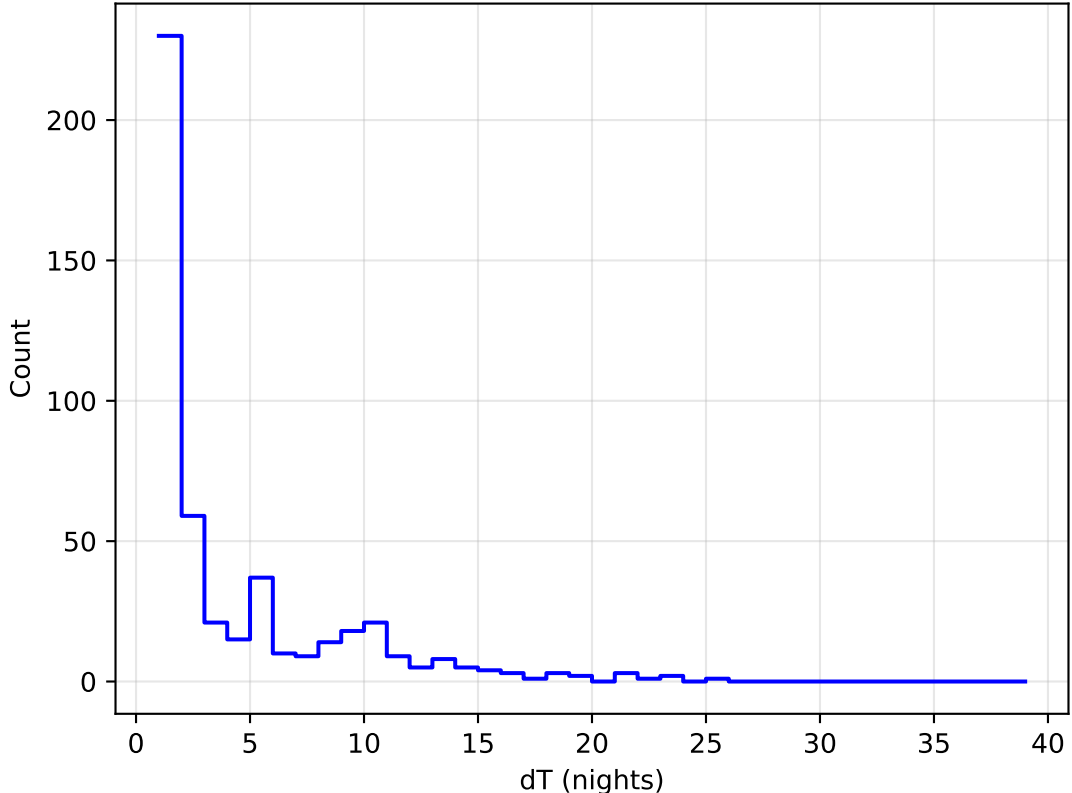
too_elab_r128_d3_ugrizy_v3.4_10yrs all bands: DD: COSMOS Delta Nights Histogram
