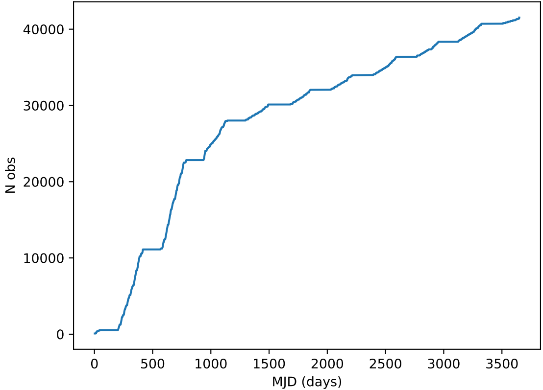
too_elab_r128_d3_ugrizy_v3.4_10yrs all bands: DD: COSMOS Cumulative NVisits
