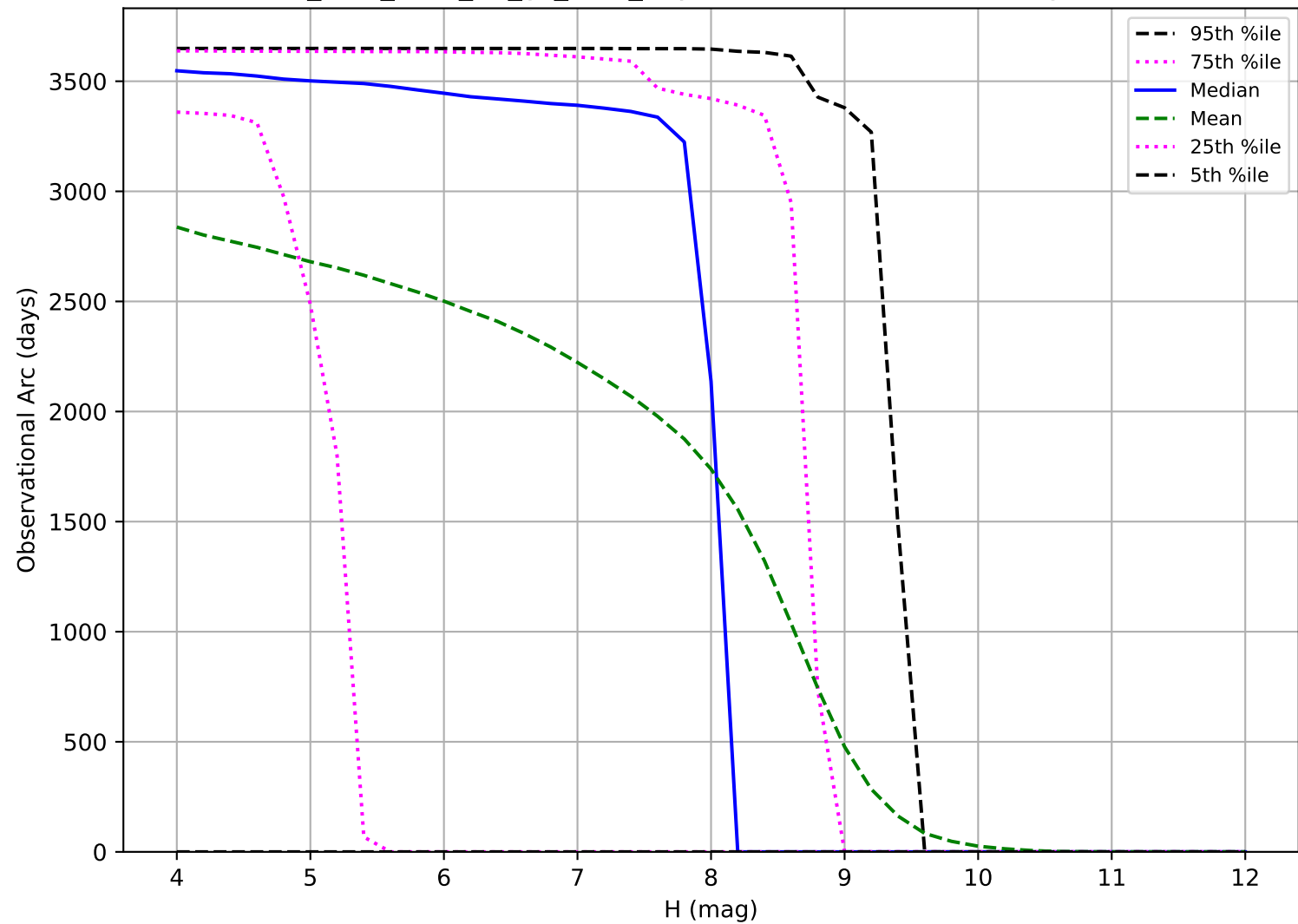
too_elab_r128_d3_gz_v3.4_10yrs: Observational Arc Length TNO
