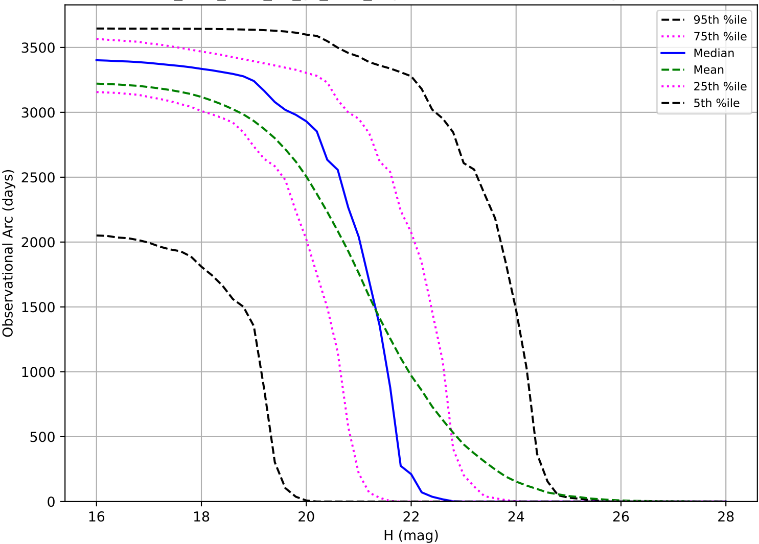
too_elab_r128_d3_gz_v3.4_10yrs: Observational Arc Length PHA
