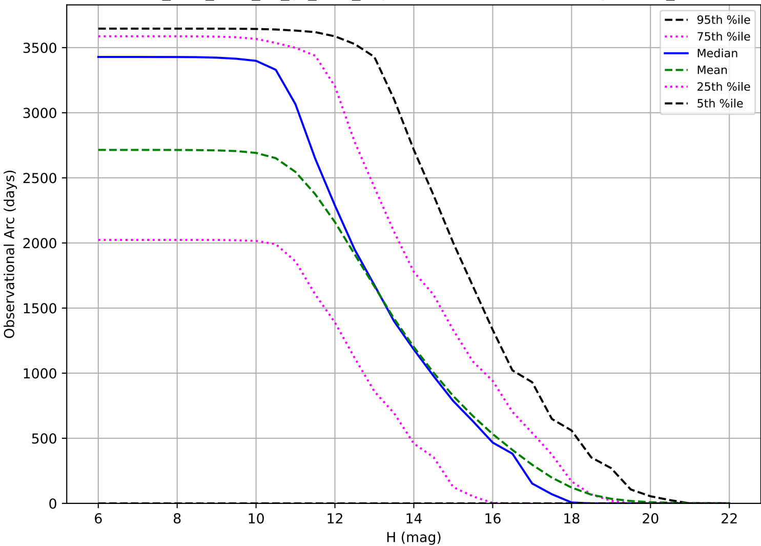
too_elab_r128_d3_gz_v3.4_10yrs: Observational Arc Length OCC_r5
